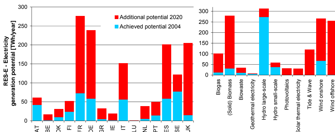
Figure 24. Achieved (2004) and additional mid-term potential 2020 for electricity from RES in the EU-15 – by country (left) and by RES-E category (right)
