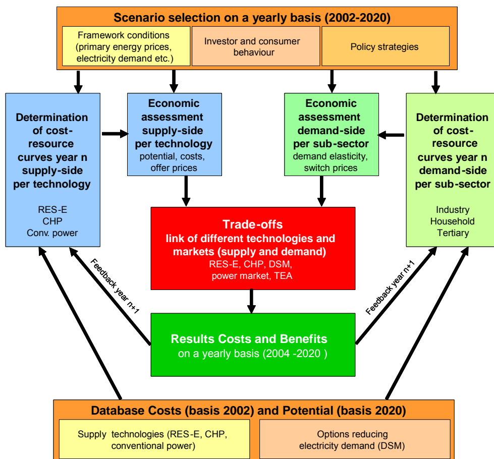
Figure 60 Overview on the computer model Green-X (electricity sector)
