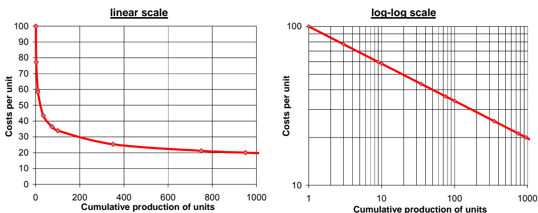
Figure 62 Characteristic run of an experience curve: On a linear (left) and on a log-log scale (right). Note: Parameter settings: LR=15\% , C_0=100 .
